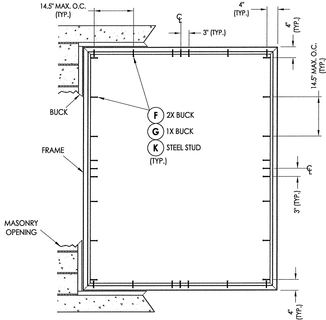
FRAME ANCHORING
