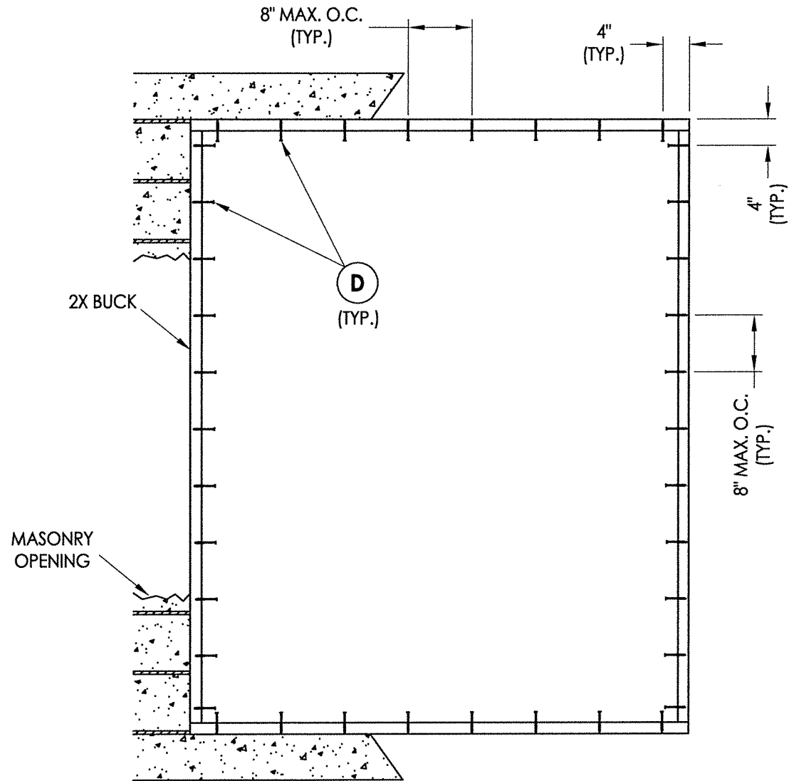
BUCK ANCHORING
